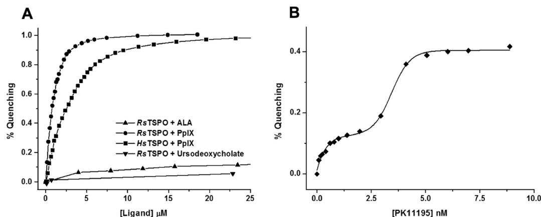
Figure 4. Binding of PpIX, ALA, and ursodeoxycholate to R s TSPO and binding of PK11195 and PpIX to H s TSPO. (A) Binding of PpIX, ALA, and ursodeoxycholate to purified R s TSPO and PpIX to partially purified H s TSPO measured with the tryptophan fluorescence quenching assay. (B) Binding of PK11195 to partially purified H s TSPO.
