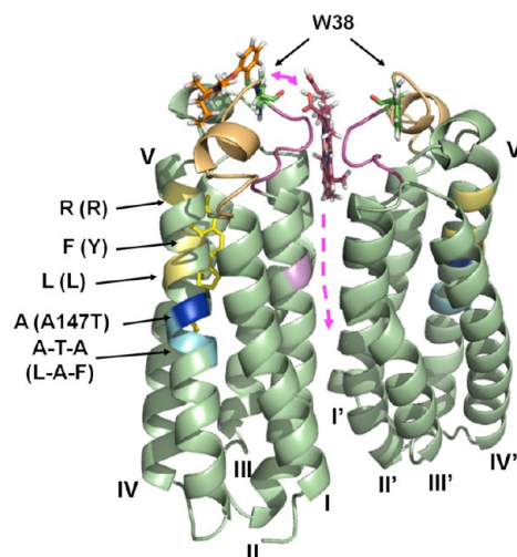
Figure 11. Proposed model of binding sites of PpIX, PK11195, and cholesterol on Rs TSPO. Structures of PK11195 and PpIX were generated with ChemDraw 3D, and that of cholesterol was taken from a published structure (PDB entry 3D4S). Note that the computational model of Rs TSPO (model 2) is generated on the basis of EM density observed in a sample without ligand. Therefore, these models may represent a closed conformation, as indicated by close association of the monomers. Ligands are manually placed into the model of Rs TSPO on one monomer, for the sake of illustration of proposed locations. Helices are labeled with Roman numerals: W38 (green sticks), PK11195 (orange sticks), PpIX (dark purple sticks), and cholesterol (yellow sticks). Highly conserved residues in the CRAC site are colored light yellow and labeled according to the Rhodobacter sequence. Corresponding residues in the human sequence are shown in parentheses. Human polymorphism residue A139 ( Rs number) is colored dark blue, while the preceding Ala-Thr-Ala sequence is colored cyan. The sequence in loop 1, before W38, that is proposed to play a role in PK11195 binding is colored light orange and corresponds to the ligand. The proposed PpIX binding sequence on loop 1 (including W44) is colored light purple, and residue W50 on helix II is colored pink. A loading and transport route for PpIX is indicated by a magenta dotted line, illustrating the potential role of the dimer in transport, which would require flexibility of the external loops.
