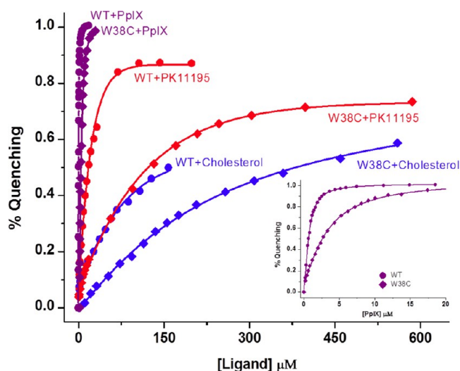
Figure 6. Binding of PpIX, PK11195, and cholesterol to purified RsTSPO (WT) and RsTSPO W38C (W38C). All binding curves were obtained and plotted as described in Materials and Methods. The inset shows a close-up of the 0–20 \mu M region to better show the binding curve of the PpIX.
